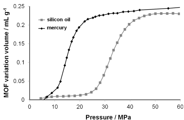
Figure 4. MOF volume variation as a function of the applied pressure of mercury and oil on the MIL-53(Al) sample during the first compression.
